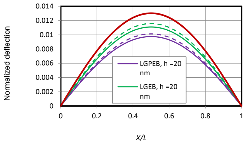
Fig. 1. Normalized deflection w/w_* of simply-supported beams with different beam thicknesses 10 nm and 20 nm
